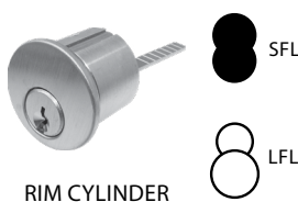
RIM CYLINDER
