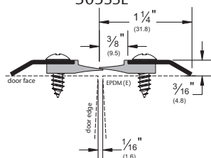
Security Bar Astragal 3572
