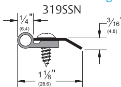
Perimeter Gasketing 319SSN
