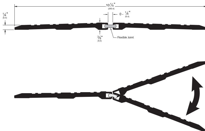
The 573x5 threshold flexes +/- 20° to allow for expansion or contraction of building materials
