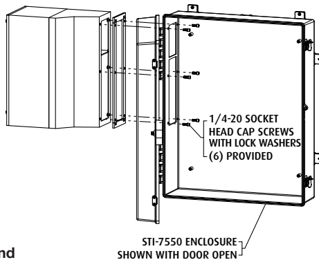
VIEW 4
