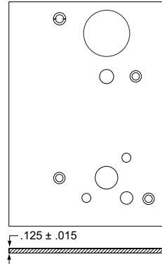
L9000 lead lining XL11-515
