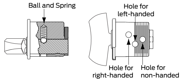
09-900 cylinder turn
