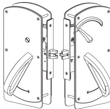
HSLR Emergency turn x thumbturn
