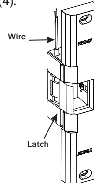
Figure 4. Position of Electric Strike for Left Hand Inswinging and Right Hand Outswinging Door
