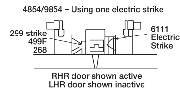
4854/9854 – Using one electric strike
