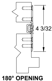
180° OPENING
