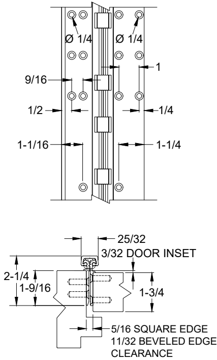
CLOSED POSITION
