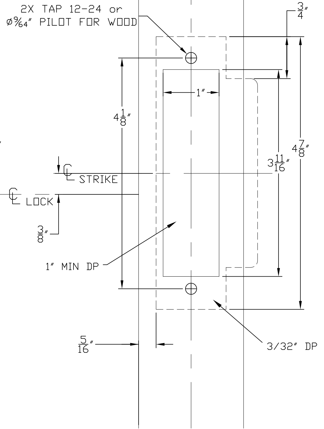
STRIKE TEMPLATE
