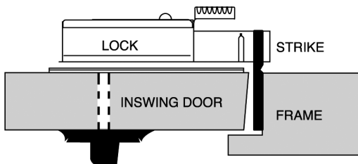
TYPE 1 Part# 114003
