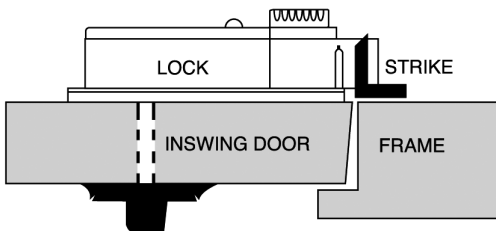
TYPE 3 Part# 114005
