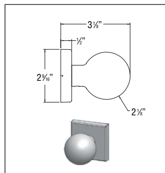
BALL KNOB (K)
